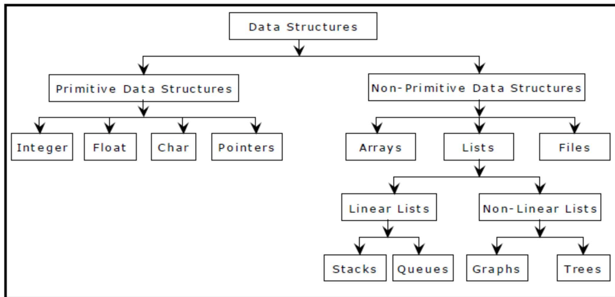
Figure 1.1. Classification of Data Structures
