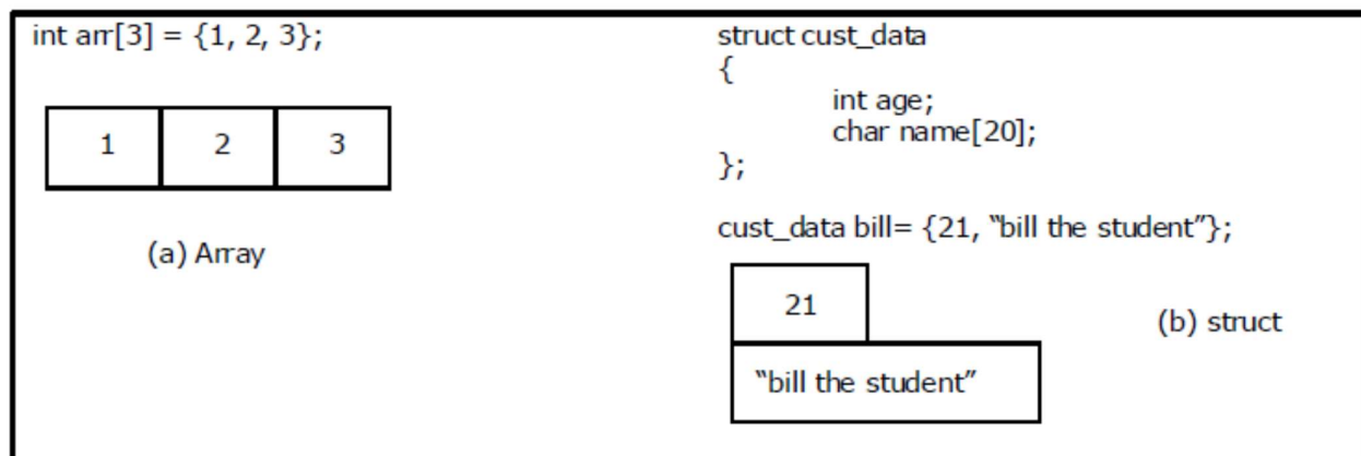
Figure 1.3 Examples of contiguous structures.
