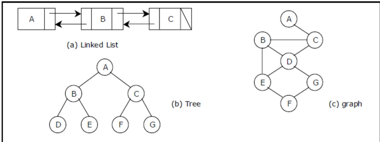
Figure 1.4. Examples of non-contiguous structures
